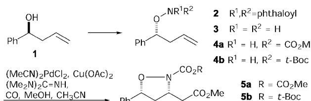
Scheme 1 Isoxazolidine synthesis.
