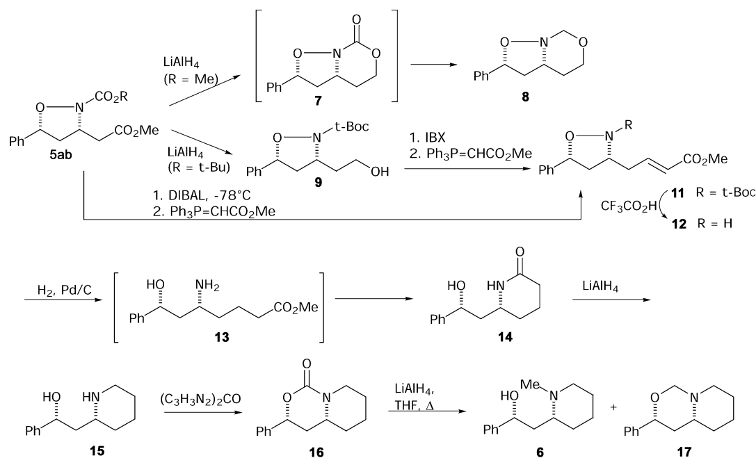
Scheme 2 Sedamine synthesis.
